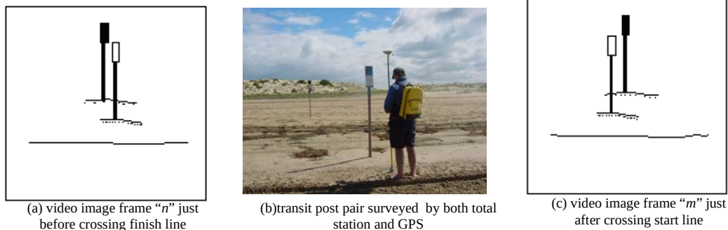
Fig. 3 Diagrammatic view of the transit posts surveyed by both conventional and GPS methods (b) and video image frames “m” and “n” at the start (c) and finish (a)
