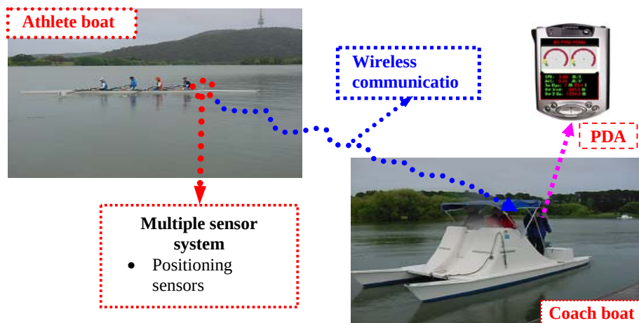
Fig. 8 Skeleton of the system structure of the "smart" rower tracking multi-sensor system with wireless communication and on-line processing functionalities.
