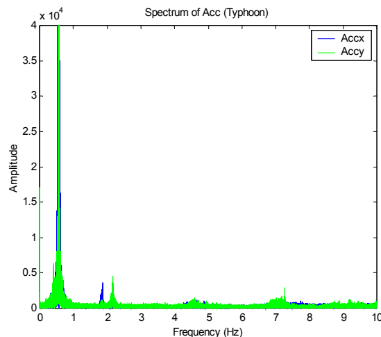
Figure 23 Overall FFT spectrums of accelerometer measurements during the typhoon.
